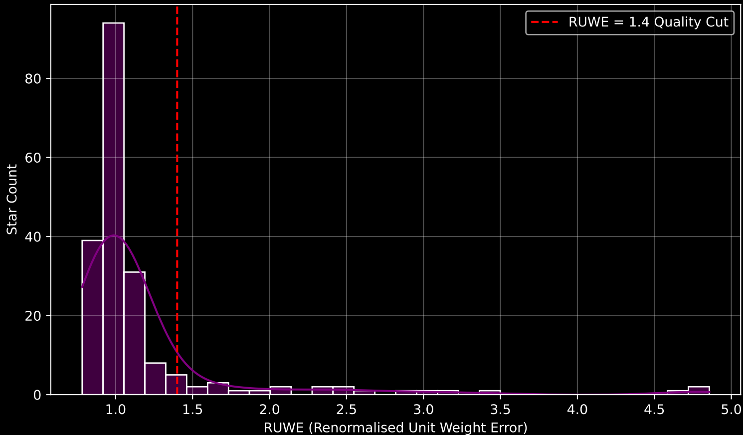
GAPOGEE DR17 Field [199+30_MGA] RUWE Distribution (n= 198)
