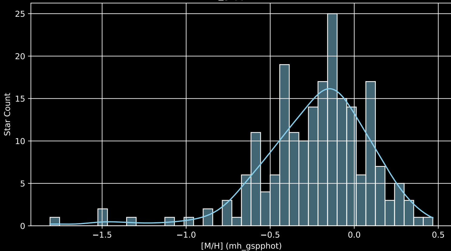
APOGEE DR17 Field: [199+30_MGA [M/H] (mh_gspphot) (n= 207)
