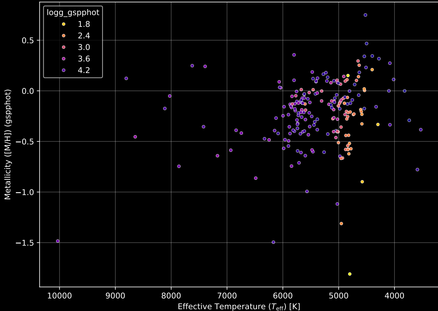
APOGEE DR17 Field: [199+30_MGA] Stellar Population Parameters (n= 208)
