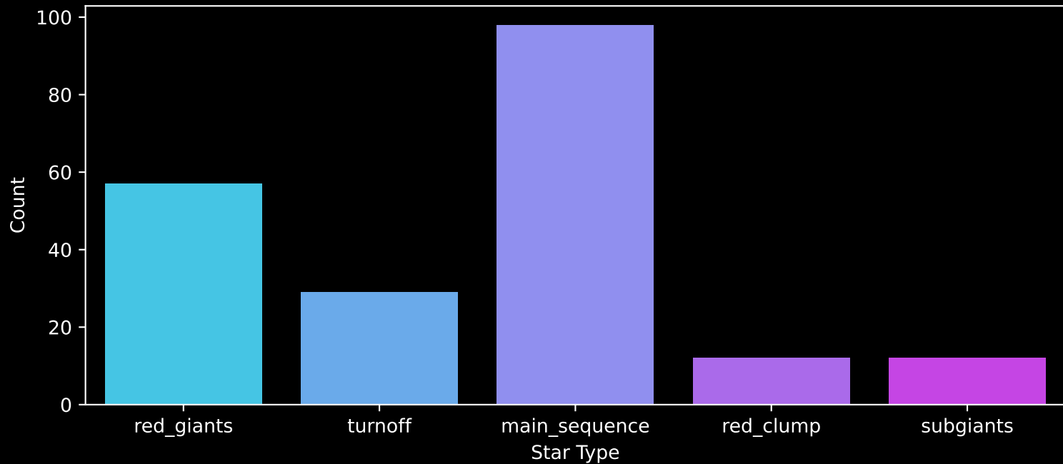
APOGEE DR17 Field: [199+30_MGA] Count plot of Star Type
