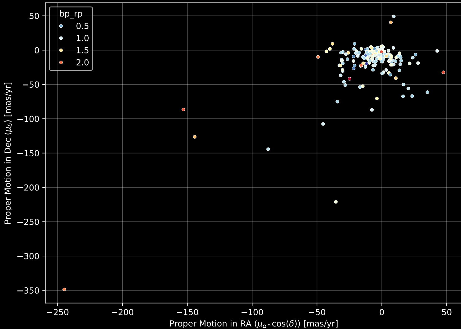
APOGEE DR17 Field: [199+30_MGA] Proper Motion Diagram (n= 208)
