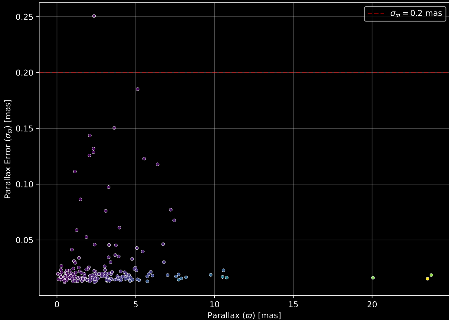
APOGEE DR17 Field: [199+30_MGA] Parallax Quality (n= 208)
